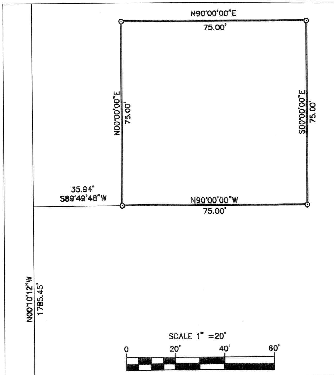
SITE DETAIL
