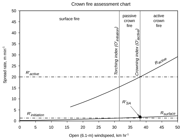
Figure 8 —The Torching and Crowning Indices can be determined graphically on a crown fire assessment chart. The open windspeed at which R_{\text{surface}} exceeds R'_{\text{initiation}} (same as I_{\text{surface}} > I'_{\text{initiation}} ) is the Torching Index (TI). The open windspeed at which R_{\text{active}} exceeds R'_{\text{active}} is the Crowning Index. A surface fire is expected at windspeeds below TI. Windspeeds greater than TI but less than CI lead to passive crowning. Active crown fire is expected at windspeeds above CI. The theoretical surface fire spread at CI ( R'_{\text{sa}} ) is shown; that quantity will be used later in the paper. Inputs: fuel model 10 (timber litter and understory, Anderson 1982), canopy base height = 1.5 m, canopy bulk density = 0.15 kg m -3 , foliar moisture content = 100 percent, normal summer surface fuel moisture condition (Rothermel 1991, table 4), and wind reduction factor = 0.15.
