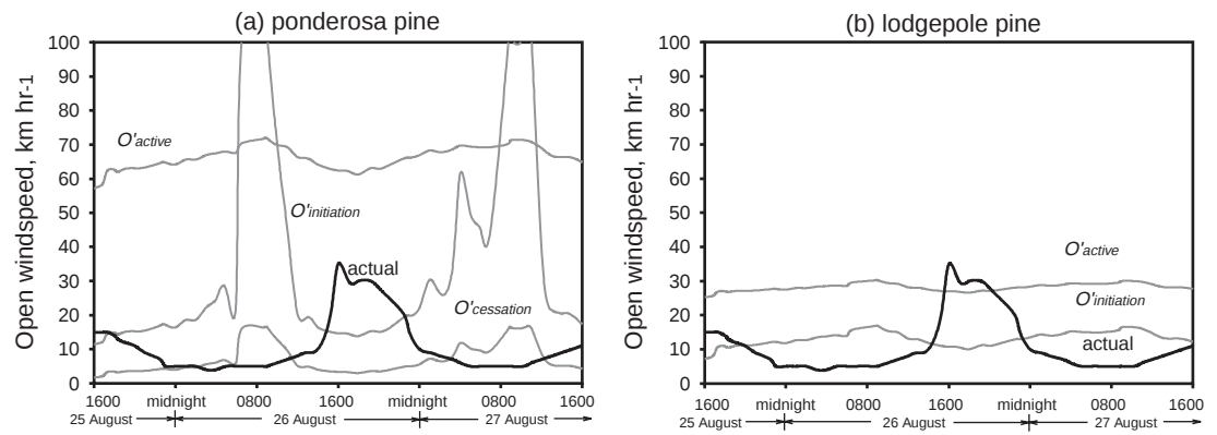
Figure 21 —Critical windspeeds for crown fire initiation, sustained active spread, and cessation for the diurnal weather depicted in figure 20 for a ponderosa pine stand (a) and lodgepole pine stand (b) on the Bitterroot National Forest, Montana. For demonstration, a hypothetical trace of “actual” windspeed is shown.
