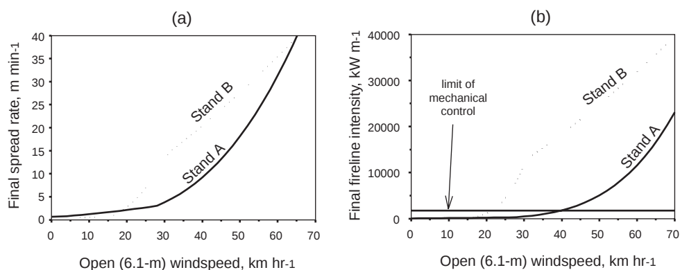
Figure 19 —Final rate of spread (a) and fireline intensity (b) for the two example stands on the Bitterroot National Forest, Montana. The limit of mechanical control (3500 kW m -1 ) is indicated.
