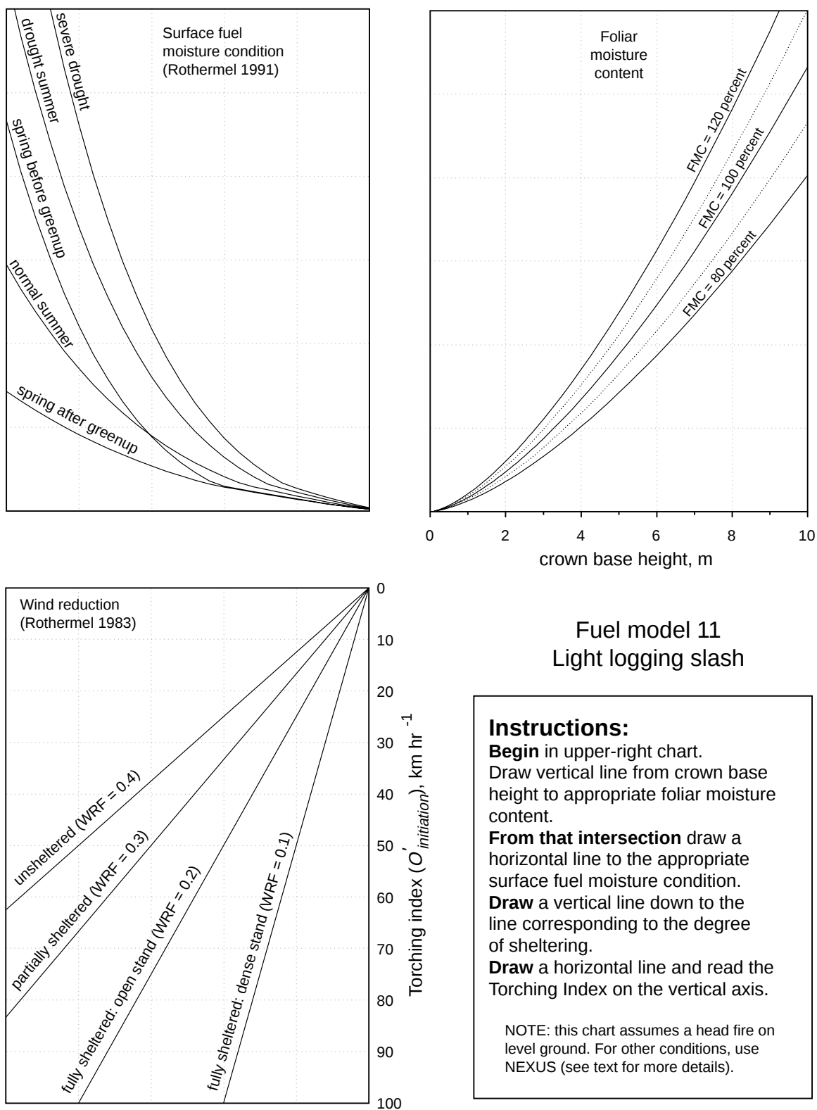
Figure D-7 —Nomogram for determining the Torching Index for fuel model 11 (light logging slash).
