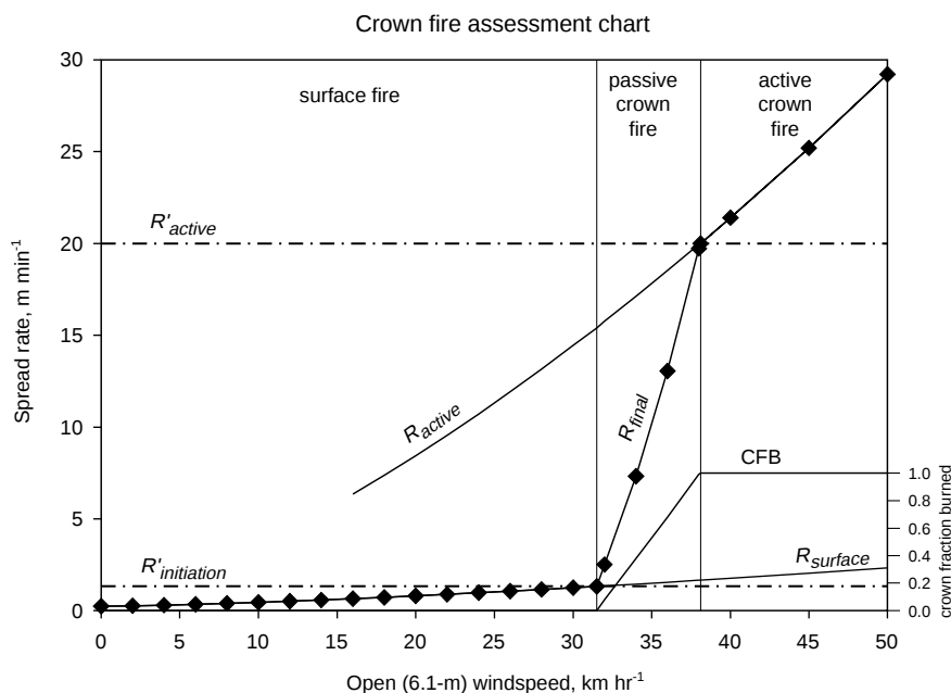
Figure 9 —Final spread rate ( R_{final} ) and crown fraction burned ( CFB ) plotted over a range of windspeeds. Crown fraction burned (right-hand Y-axis) is 0 until windspeed reaches the TI, then increases to 1 where windspeed reaches CI. In the surface fire region, R_{final} = R_{surface} . In the passive crown fire region, final spread rate is scaled between R_{surface} and R_{active} . In the active crown fire region, R_{final} = R_{active} . Inputs: fuel model 10 (timber litter and understory, Anderson 1982), canopy base height = 1.5 m, canopy bulk density = 0.15 kg m -3 , foliar moisture content = 100 percent, normal summer surface fuel moisture condition (Rothermel 1991a, table 4), and wind reduction factor = 0.15.
