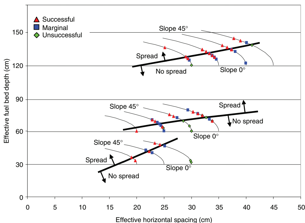
Fig. 6. Regression thresholds for spread in discontinuous fuel beds (bold black lines) are plotted by effective fuel-bed depth ( Z + \text{gap} \times \sin(\text{slope}) ) and effective horizontal spacing ( \text{gap} \times \cos(\text{slope}) ) where the ‘gap’ represents the separation distance between fuel rows as measured parallel with the surface plane of the platform (see Table 1 for summary of experimental data and Table 2 for regression statistics). For a given fuel depth category, experimental fires would successfully spread above these thresholds but not spread below them. Deeper beds and narrower horizontal gaps facilitated spread. The potential range of experimentally controlled variables is indicated by the curving fine lines that delineate effect of slope changes ( 0^\circ to 45^\circ ) for the depth and spacing combinations. Coloured points represent the results of individual burns in terms of their success in producing fire spread the entire length of the bed (see text under Methods).
