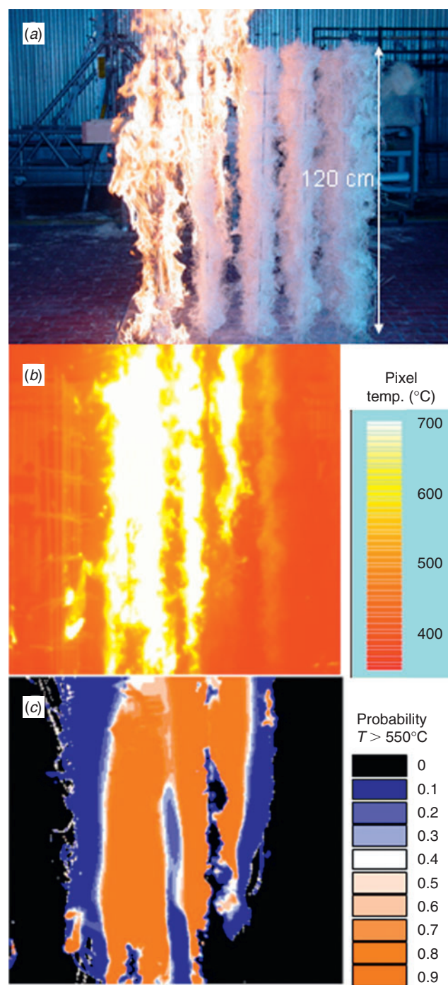
Fig. 2. Images of an experimental fire burning left to right across a discontinuous fuel bed. Visible image (a) and thermal image (b) show non-steady flame behaviour at the leading edge of the fire. This non-steady flame behaviour was characterised by a probability of flame presence (temperature greater than 550°C) over 8 s of 120-Hz thermal images.
