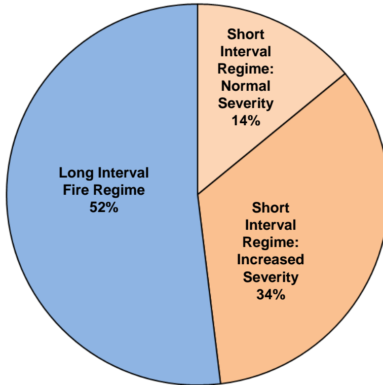
Figure 32 – Trend toward increased fire susceptibility for short-interval fire regimes of the Pacific Northwest. 1 Many sources show that the scale of predicted change in fire severity for fire regime 1 sites has been enormous (Hessburg et al. 2005, Hann et al. 1997, Quigley et al. 1996, and other sources in the References section). When considering the 47 million acres of federal lands in the Pacific Northwest, which are administered by the Bureau of Indian Affairs, Bureau of Land Management, National Park Service, U.S. Fish and Wildlife Service, and U.S. Forest Service, about 48% of the total acreage can be assigned to a short-interval fire regime (primarily fire regimes 1 and 2). Of this dry-site acreage, 71 percent (16 million acres, or 34% of the total acreage) currently has a higher predicted fire severity (stand-replacing) than would have existed historically (stand-maintaining severity). When the General Accounting Office evaluated catastrophic fire risk for the western U.S., its report concluded that “the most extensive and serious problem related to the health of national forests in the interior West is the over-accumulation of vegetation.” GAO estimated that about 39 million acres of national forests in the West have high fire risk due to excessive fuel buildup; they estimated that $12 billion would be needed between 1995 and 2015 to reduce excess fuel accumulations, an average expenditure of $725 million annually (GAO 1999).
