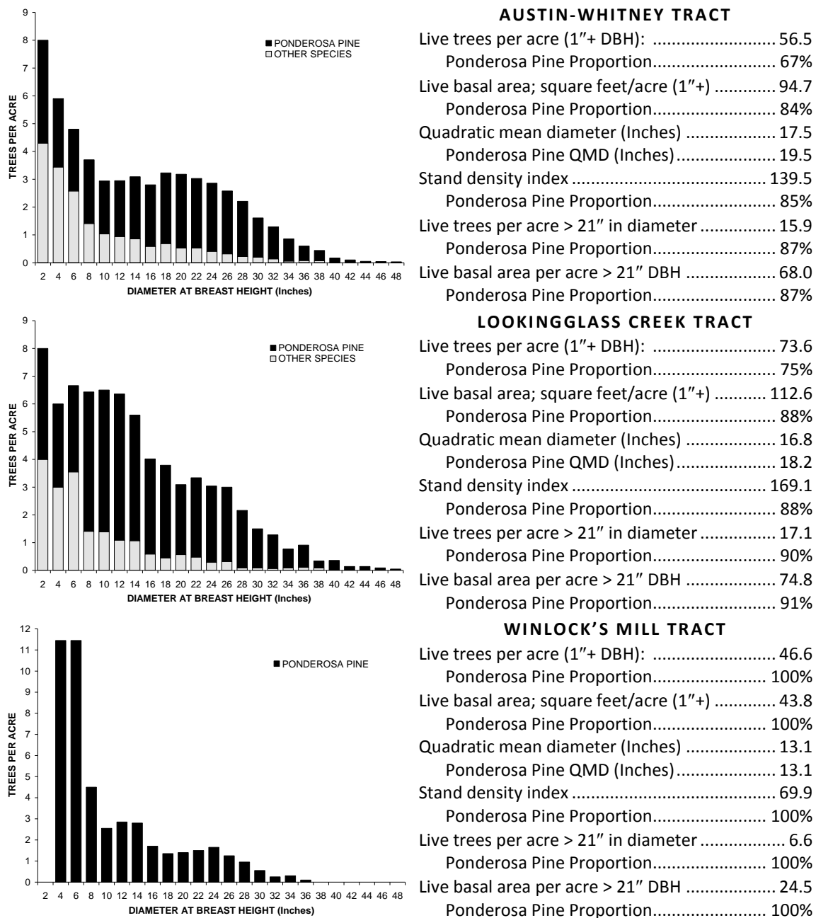
Figure 18 – Selected stand attributes for three forested tracts in the Blue Mountains of northeastern Oregon (adapted from Powell 1999). This data was derived from relatively large sample areas measured in 1910 or 1911 (sampled areas were 258½ acres for Austin-Whitney, 44 acres for Lookingglass Creek, and 20 acres for Winlock’s Mill). Data sources were Bright (1912) and Munger (1912, 1917).
