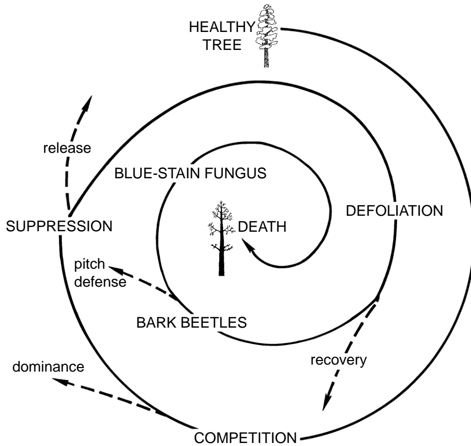
Figure 24 – Death spiral for a Douglas-fir tree in the Blue Mountains (adapted from Franklin et al. 1987). In this death spiral example, a slightly taller tree suppresses a shorter but otherwise healthy tree. If not released from competition, the suppressed tree is predisposed to attack by defoliators. Once partially defoliated, the weakened tree is attractive to bark beetles such as Douglas-fir beetle (Wickman 1978) that carry blue-stain fungus. The fungus blocks water and sap movement in the tree and causes foliage desiccation. In this model of tree decline, suppression is a predisposing stressor; bark beetles and defoliation function as culminating or inciting stressors (Pedersen 1998).
