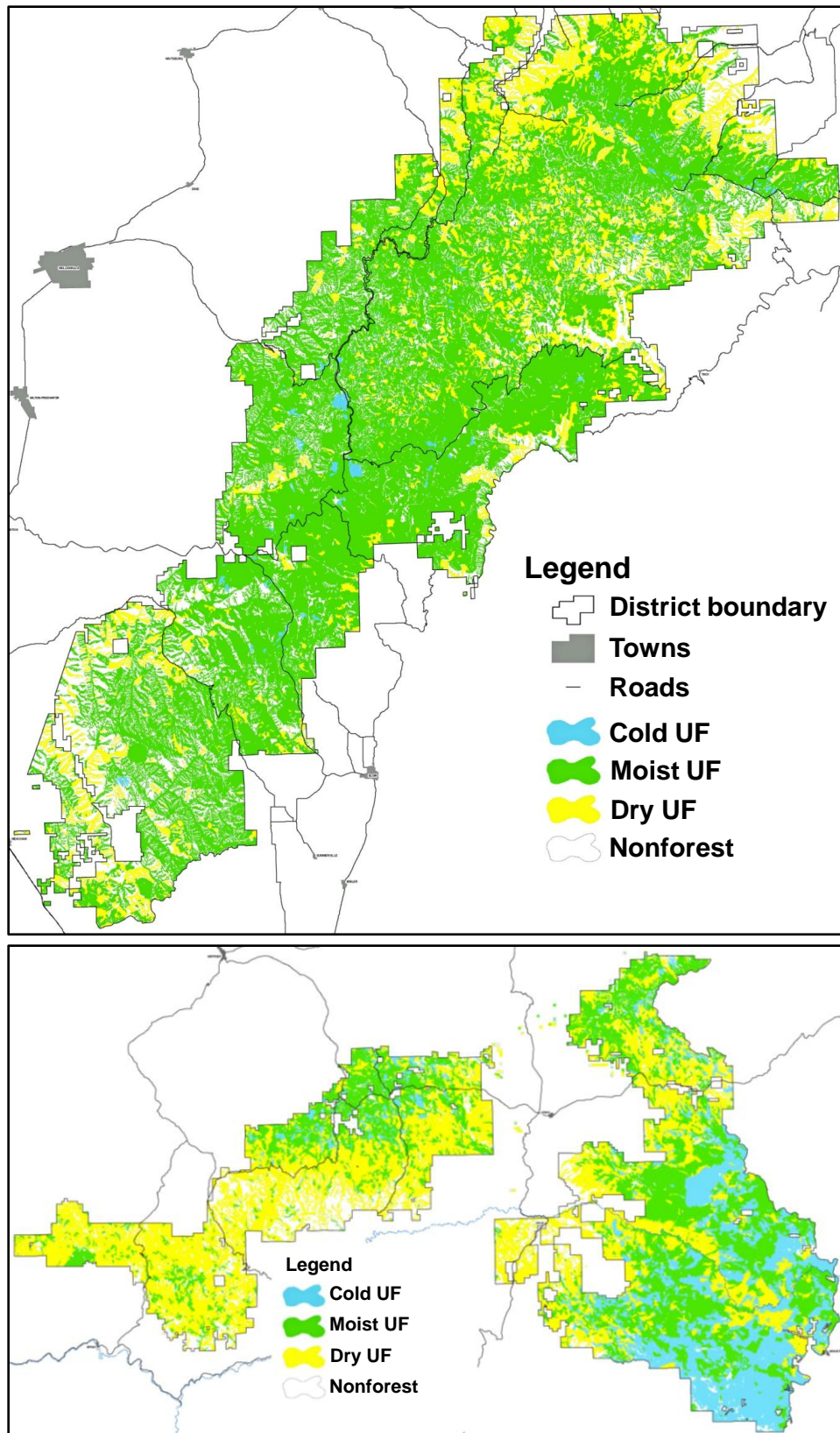
Figure 2 – Distribution of the dry upland forest (UF) potential vegetation group on the Umatilla National Forest.
